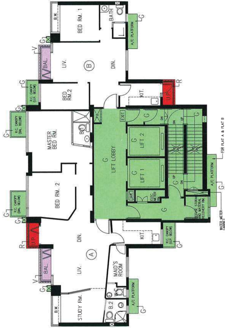
33/F PLAN (PENTHOUSE)
