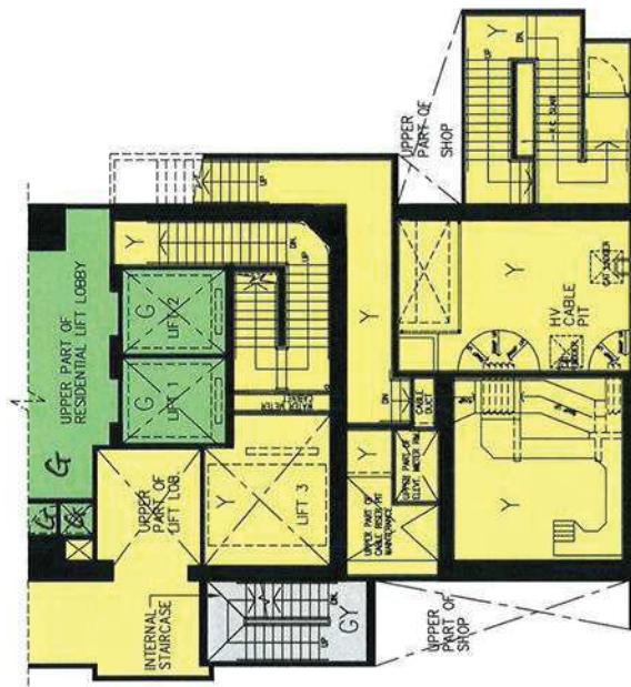
PART PLAN FOR HV CABLE PIT AT LEVEL 7.850
