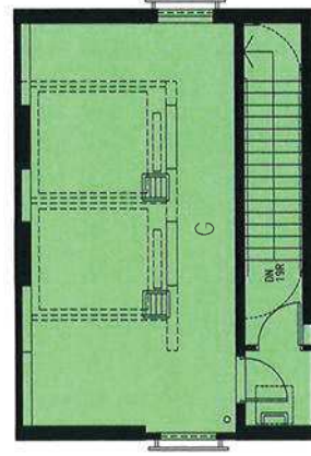
LIFT MACHINE ROOM PLAN
